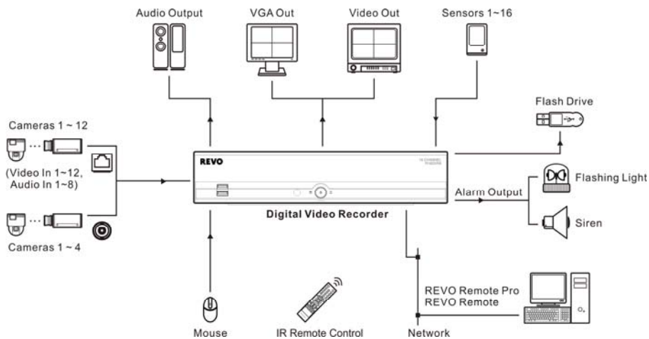
Typical DVR installation
