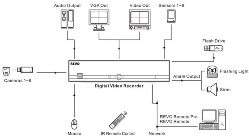
Typical DVR installation
