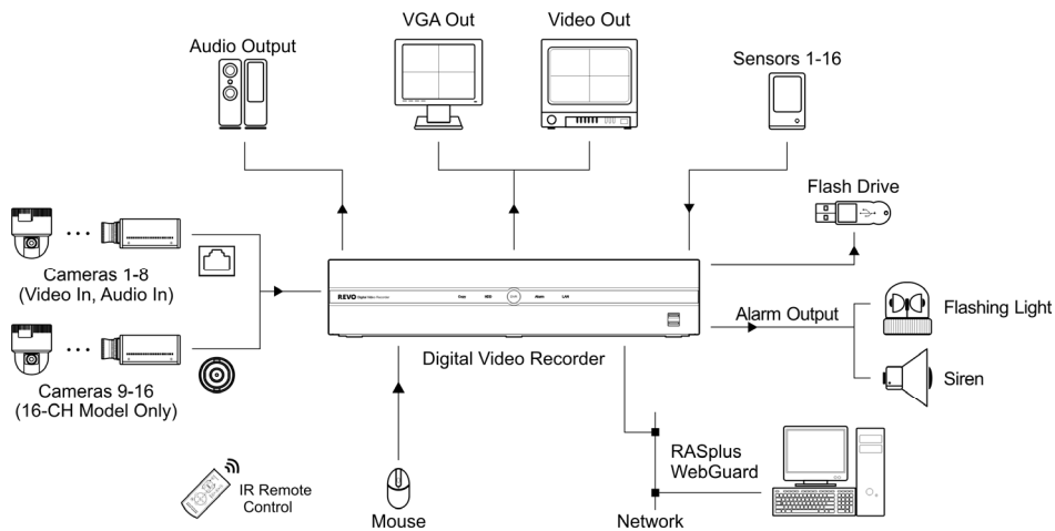
Typical DVR installation
