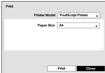
Figure 57: Print screen.
