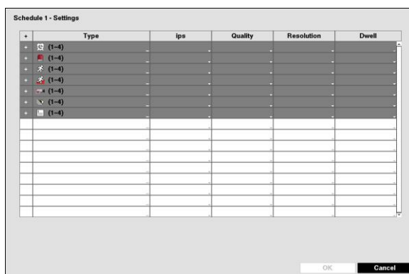
Figure 16: Schedule – Settings (Advanced Mode) setup screen.
